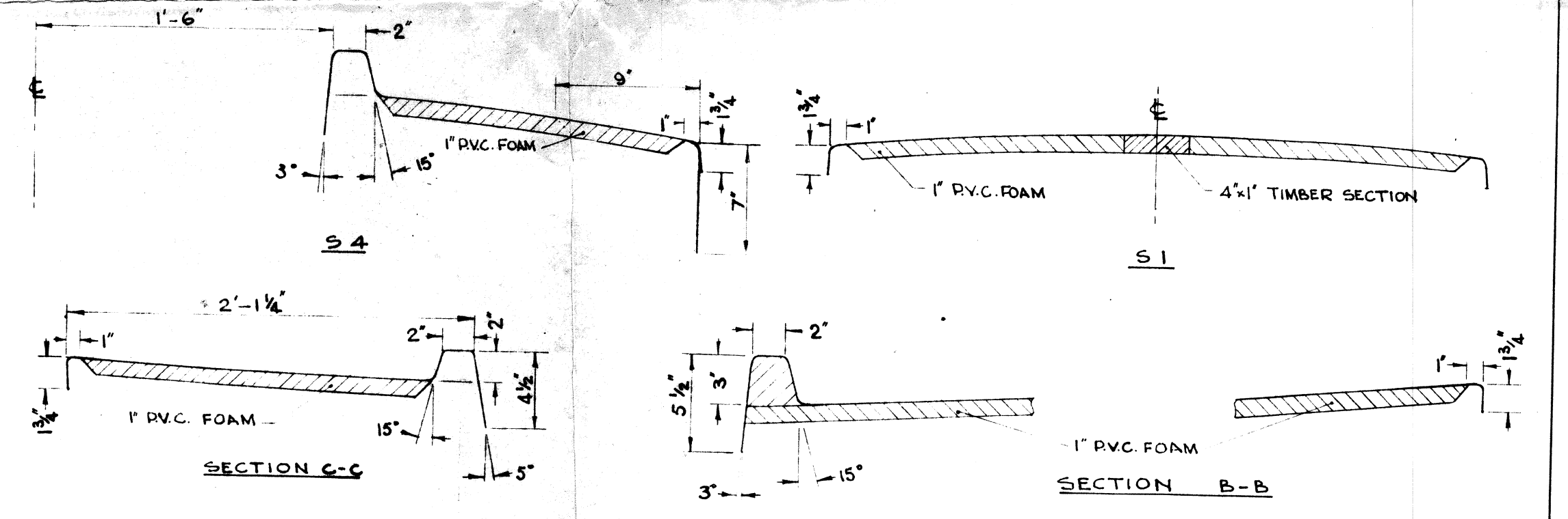
DECK SECTIONS SCALE 1/2" = 1'-0"
